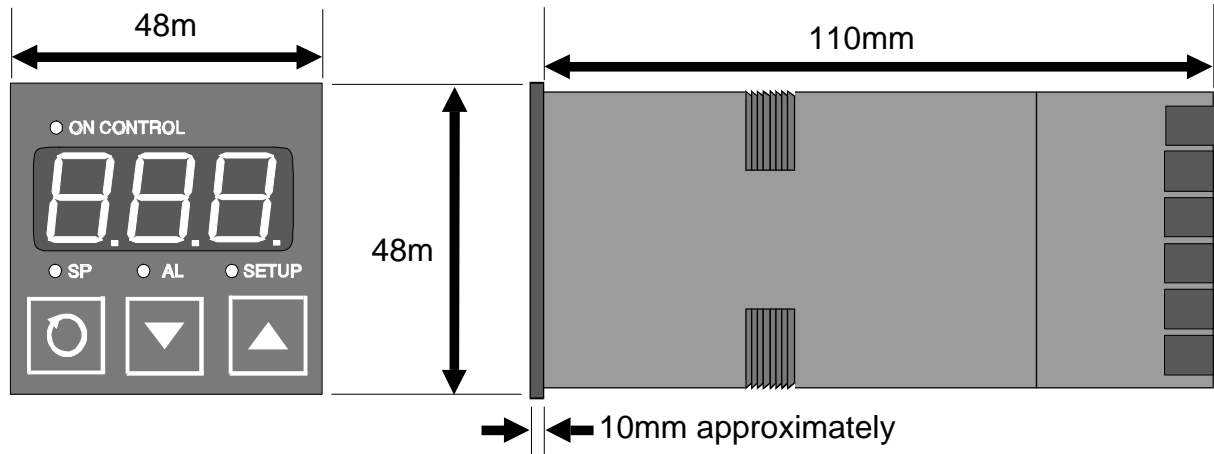
Figure 2-2 Main Dimensions
