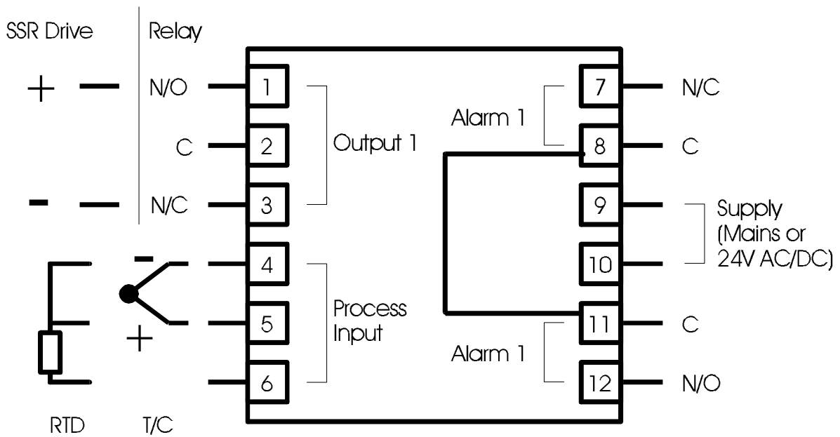
Figure 3-1 Rear Terminals
