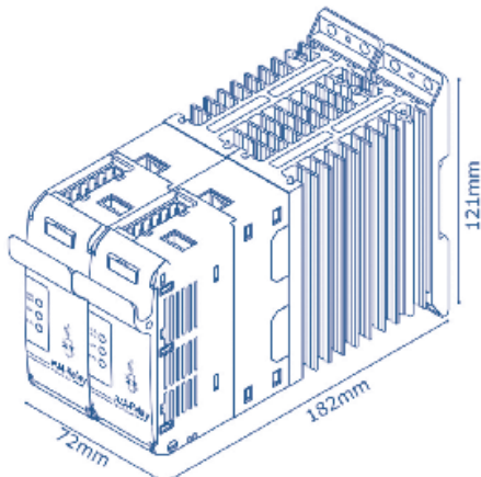
W 72 mm. - H 121 mm. - D 185 mm. - kg. 1,22 Relay S, with Fuse Holder 30A ÷ 40A
