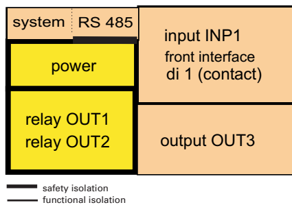
Fig. 1: Galvanic isolation
