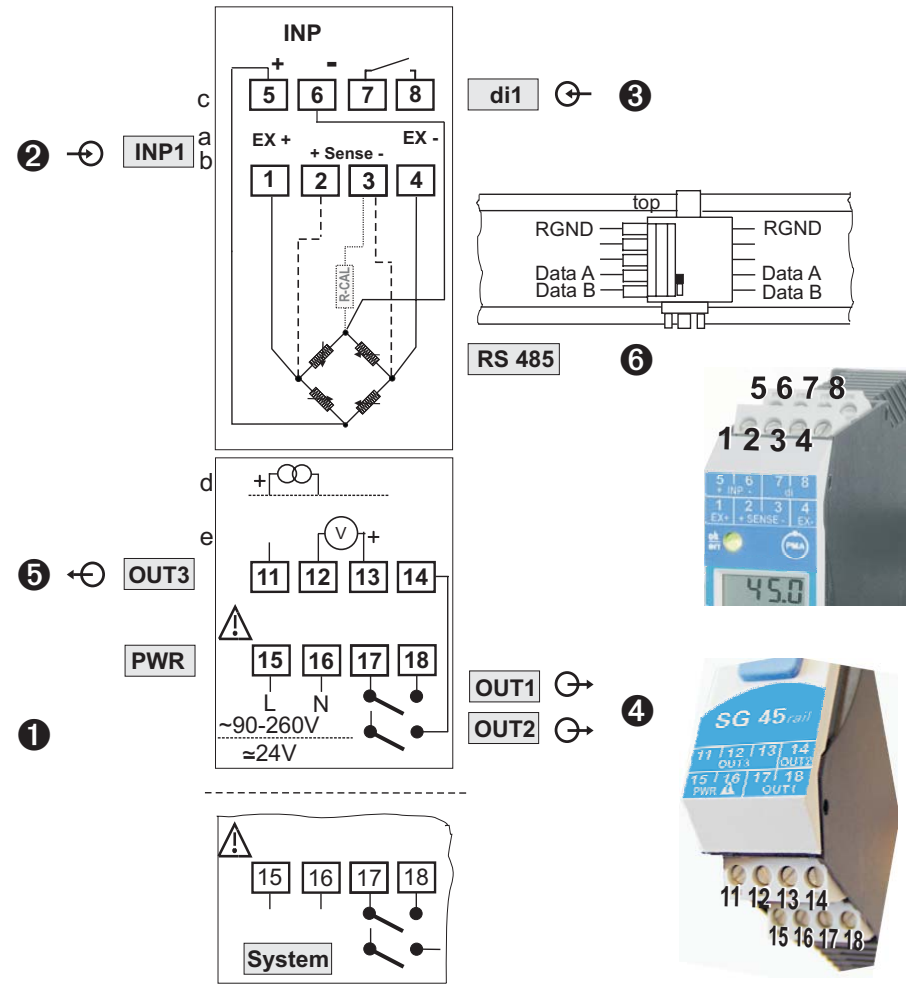
Fig.2: Electrical connections SG 45
