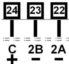
Figure 29. Plug-in Module Slot 2 – Dual SSR Driver Module
