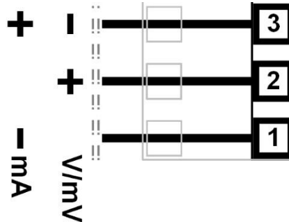
Figure 13. Input 1 - DC Volt, mV & mA Connections
