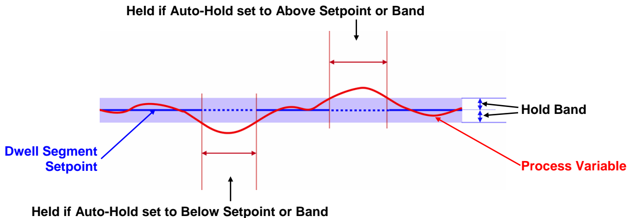
Figure 52. Auto-Hold on a Dwell Segment
