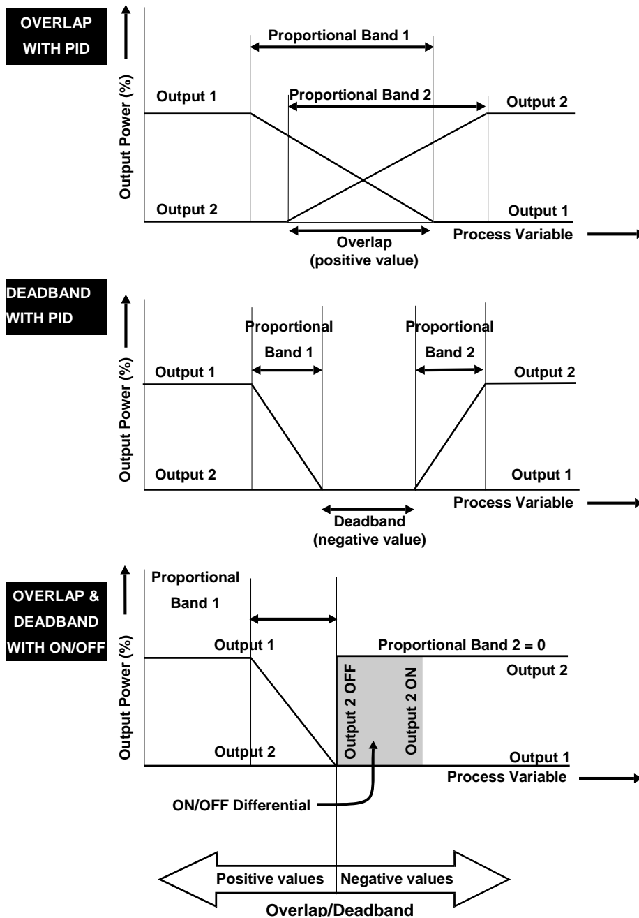
Figure 65. Overlap/Deadband
